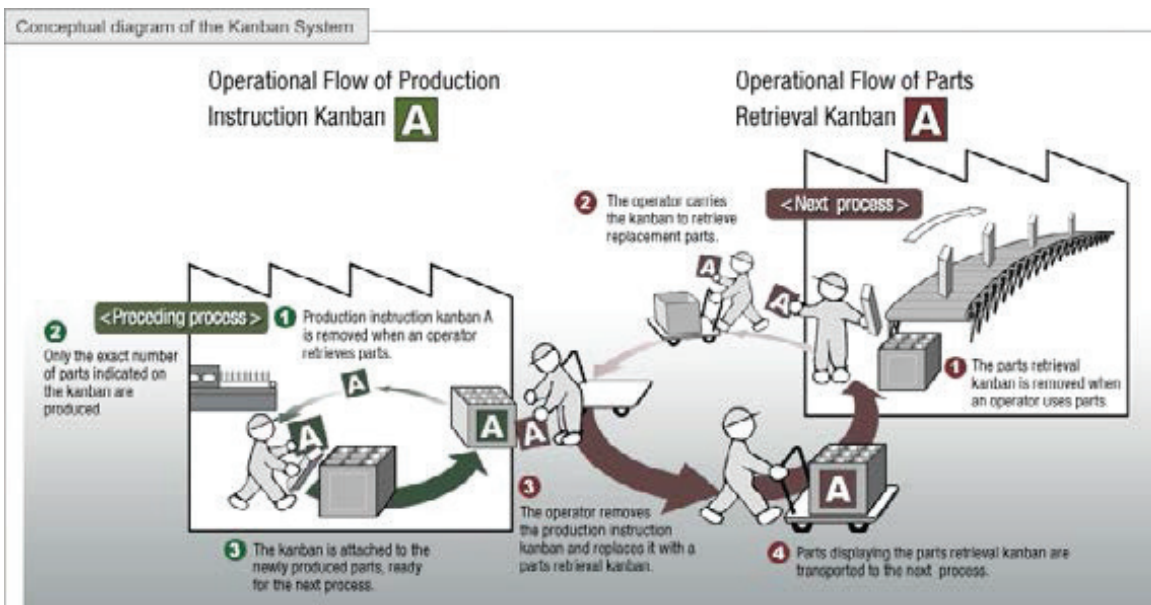
Figure 17: Kanban System
